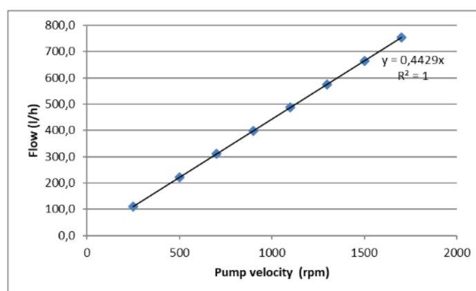
Figure 11. Results of field measurements carried out to determine the flow repeatability at the persiltaltic pump SPX 25 from Salobo plant
