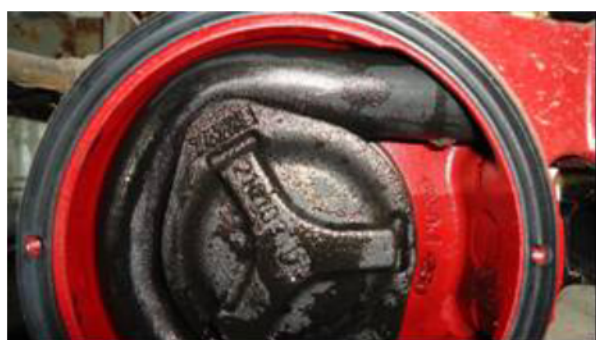
Figure 7: Peristaltic pump hose after 8 months of operation
